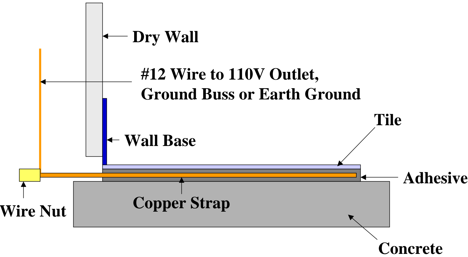
Suggested Grounding Method
