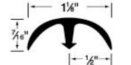
ACC04 Snap-Down Divider 1 1/8" 20 pieces/carton, Length: 12'
