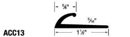
ACC13 Carpet Cove Cap 20 pieces/carton, Length 12'
