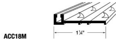
ACC18M Metal Track with Pins (aluminum finish, no color) 20 pieces/carton, Length: 12'
